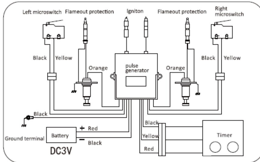
Figure 5a Internal wiring diagram of gas hob with a timing function (for reference only)
