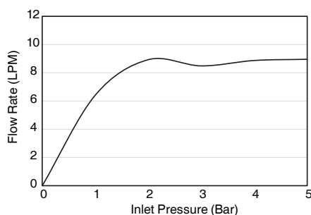
Flow Curve (Showerhead)
