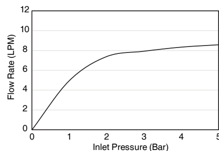
Flow Curve (Handshower)
